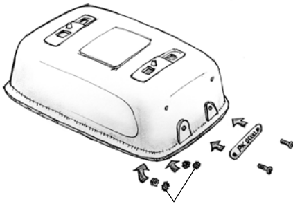
Sawtooth Washers
