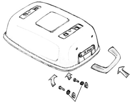
Sawtooth Washers
